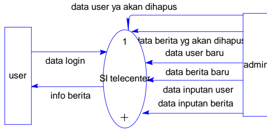
Gambar 1. DFD level 0 Telecenter
