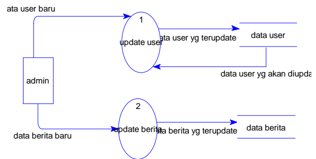
Gambar 5. DFD level 1.3 Sistem Telecenter
