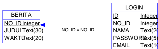
Gambar 8. PDM (Physical Data Model)
