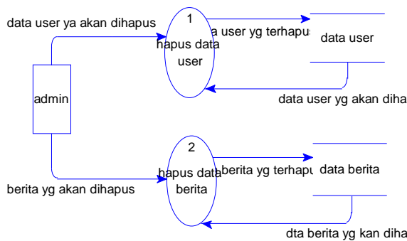
Gambar 6. DFD level 1.4 Sistem Telecenter
