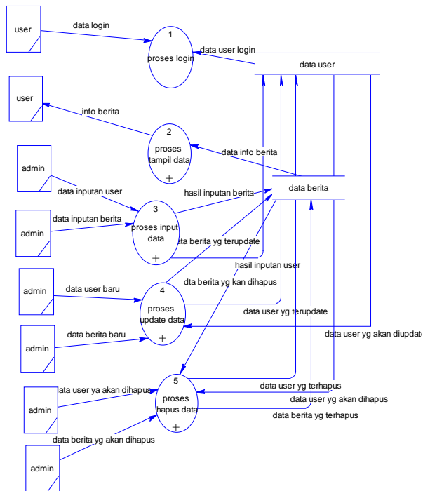
Gambar 2. DFD level 1 Telecenter
