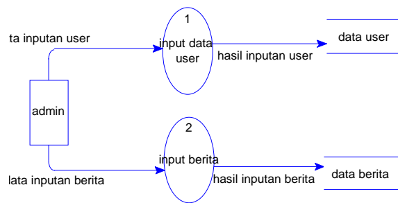
Gambar 4. DFD level 1.2 Sistem Telecenter
