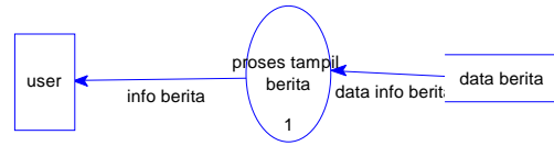
Gambar 3. DFD level 1.1 Sistem Telecenter
